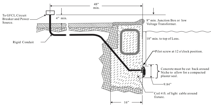
Installation Diagram for NS75 / NS150 Series
