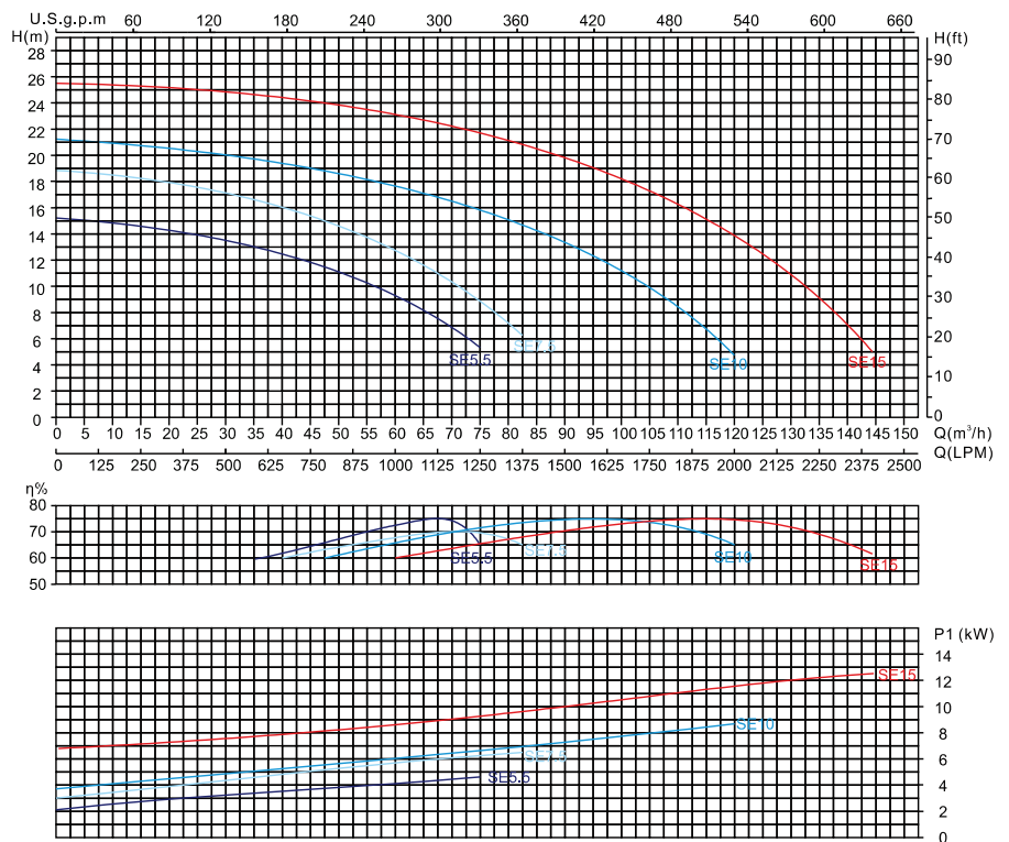
Flow curve info based on 380V/50Hz motor
